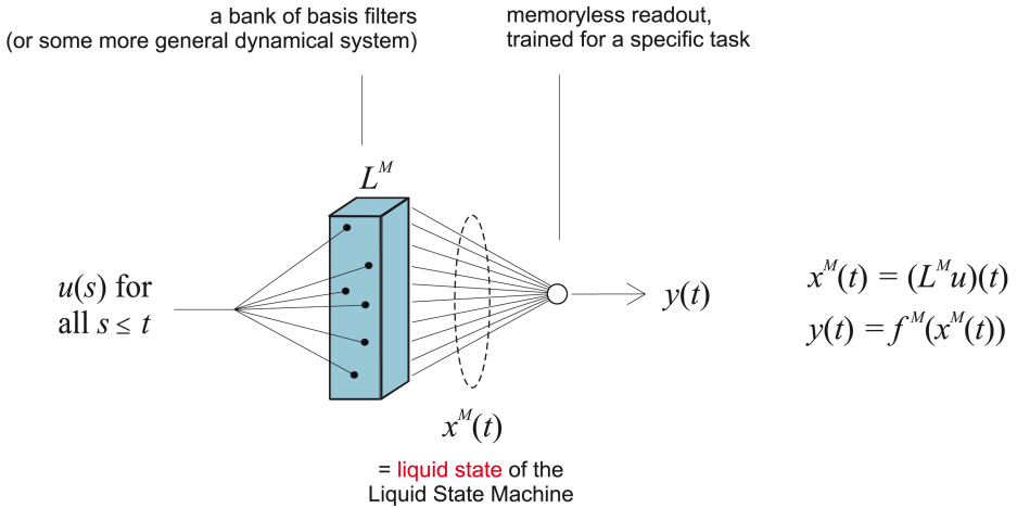
Fig. 1. Structure of a Liquid State Machine (LSM) M , which transforms input streams u(\cdot) into output streams y(\cdot) . If L^M is a bank of k basis filters, the “liquid state” x^M(t) \in \mathbb{R}^k is the output of those k filters at time t . If L^M is a more general dynamical system, x^M(t) is that part of its current internal state that is “visible” for a readout.
