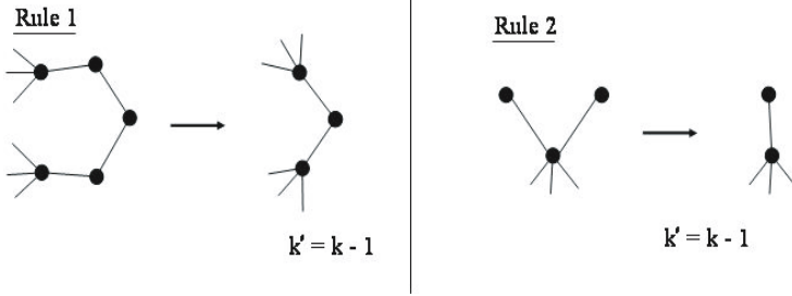
Fig. 3. Reduction rules for maximum independent set
