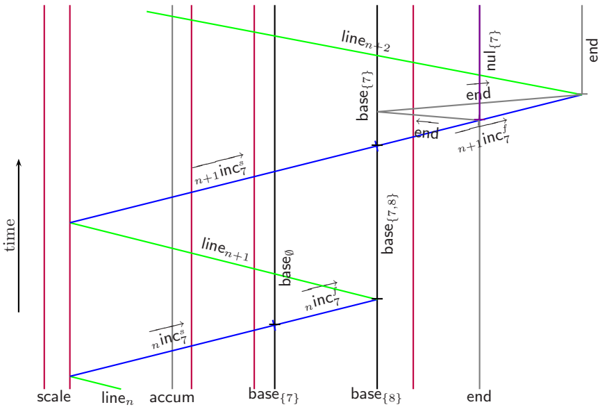
Fig. 4. Example of register updating: n:\text{inc } A_7 n+1:\text{inc } A_8
