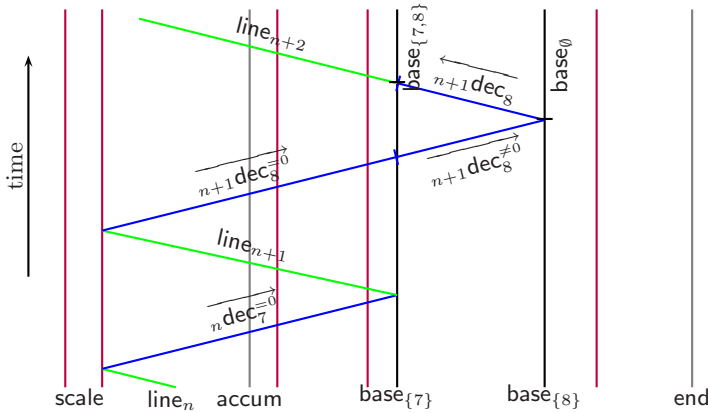
Fig. 3. Example of register updating: \begin{matrix} n: \text{dec } A_7 \\ n+1: \text{dec } A_8 \end{matrix}
