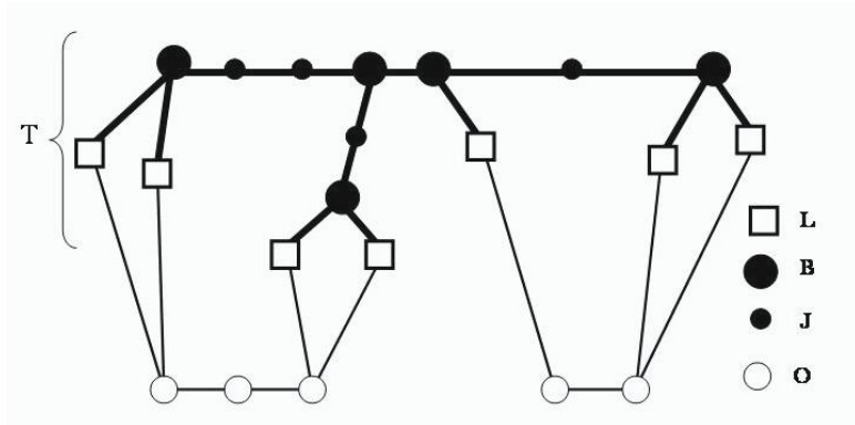
Fig. 2. The witness tree and various sets of vertices
